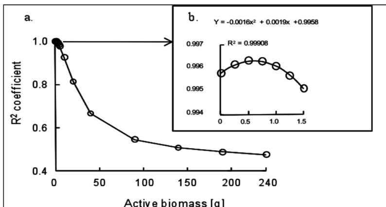
Figure 1: Logistic model fitting against numerically-partitioned active biomass (a), the peak as at 0.60g with the highest R^2 coefficient was 0.9963 (b).
