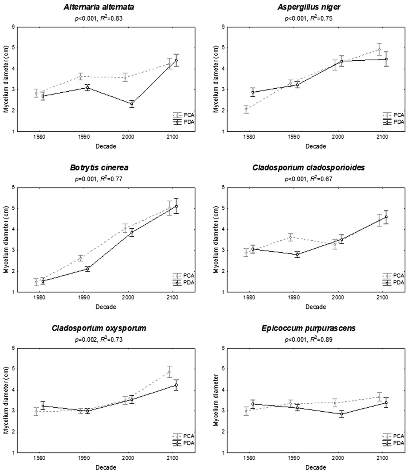
Fig. 1 Differences (full factorial ANOVA) in fungal growth ( dependent variable ) between different nutrient levels, PCA and PDA, and temperature decadal averages during 1980–2010 and 2100 projection (categorical predictors; X axis ) and over sampling time (covariate). Fungal growth ( Y axis ) is expressed as mycelial diameter in centimeter. Standard
